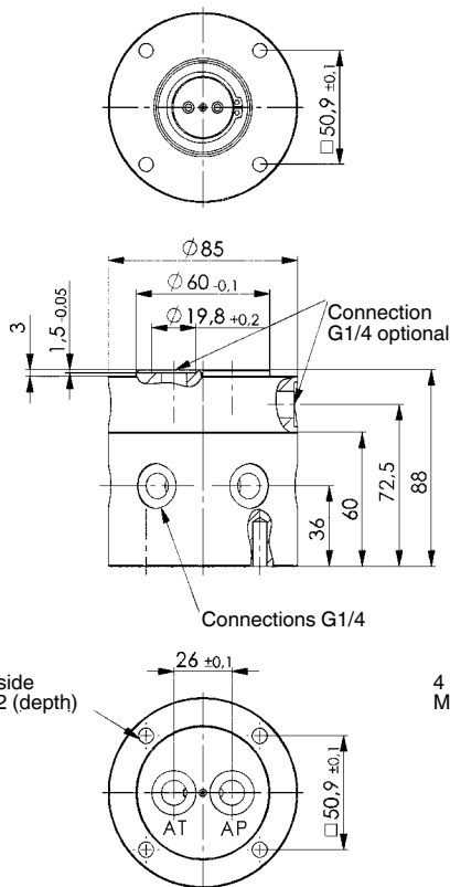
No. 6992H-11-06
