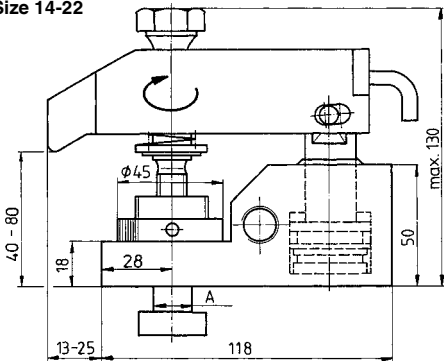
Size 14-22
