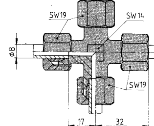
No. 6994-09 Cross-pattern bolting
