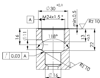
Mounting hole
