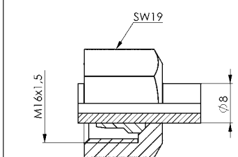
No. 6994-17 Union nut with cutting ring
