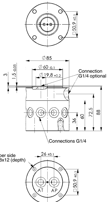
No. 6992H-11-10
